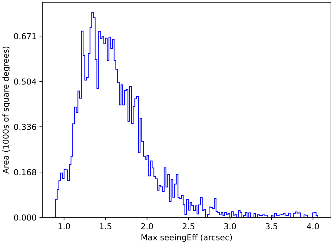
too_elab_r256_d3_griz_v3.4_10yrs Yr 1 g band: Max seeingEff
