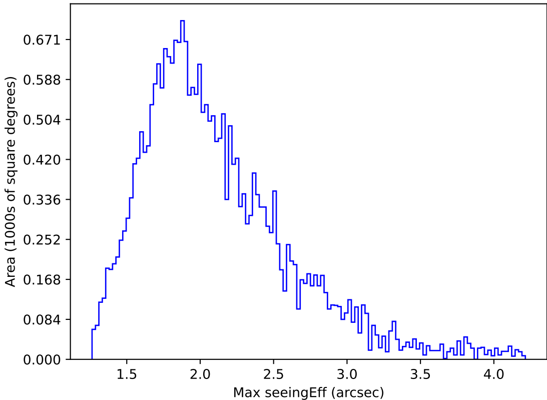
too_elab_r256_d3_griz_v3.4_10yrs Yr 1 all bands: Max seeingEff
