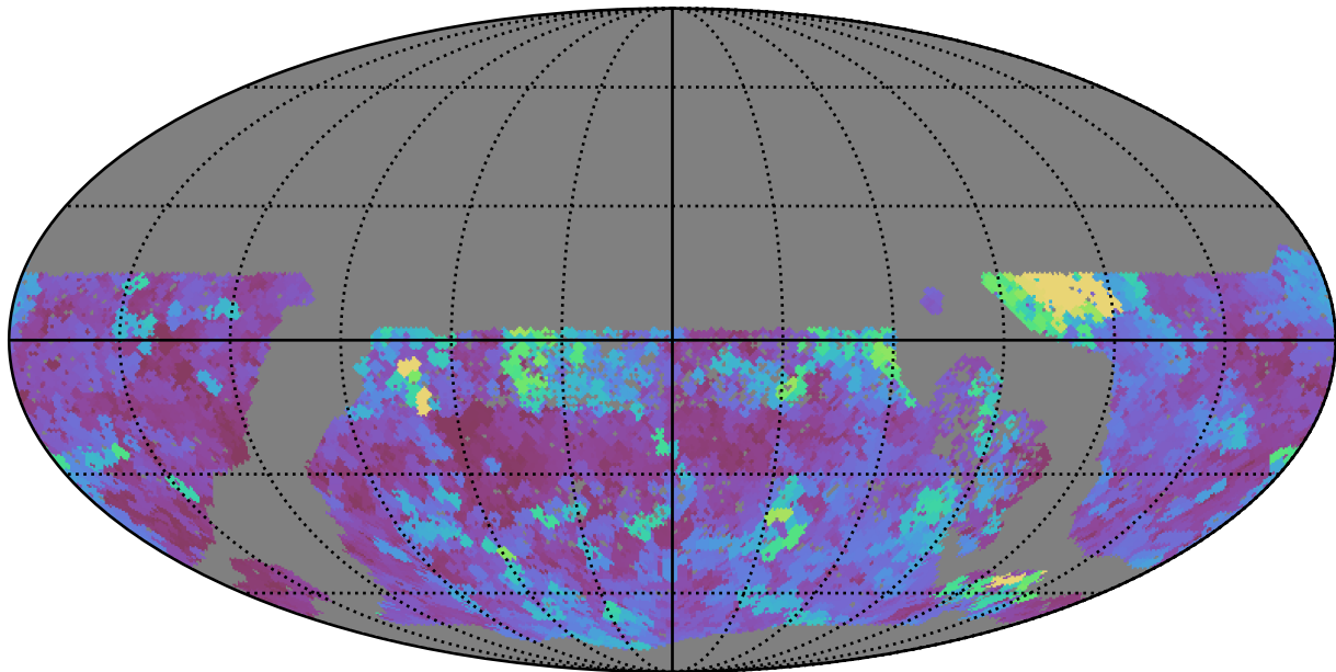
too_elab_r256_d3_griz_v3.4_10yrs WFD u band: Max seeingEff
