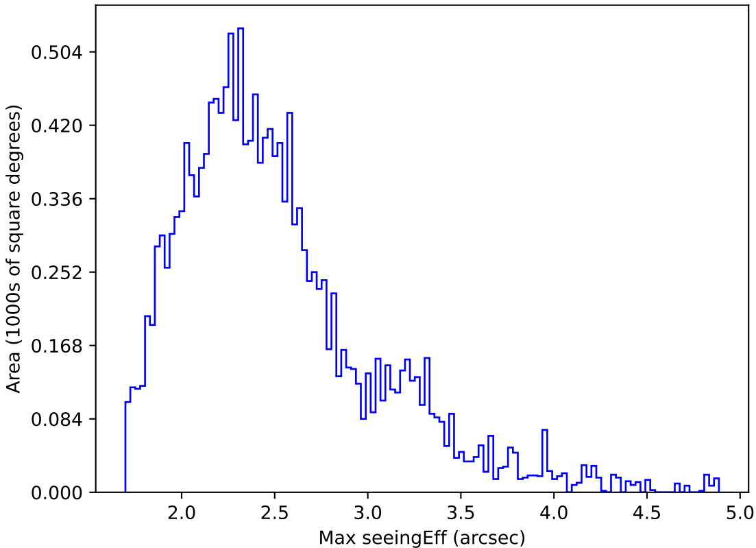
too_elab_r256_d3_griz_v3.4_10yrs WFD u band: Max seeingEff
