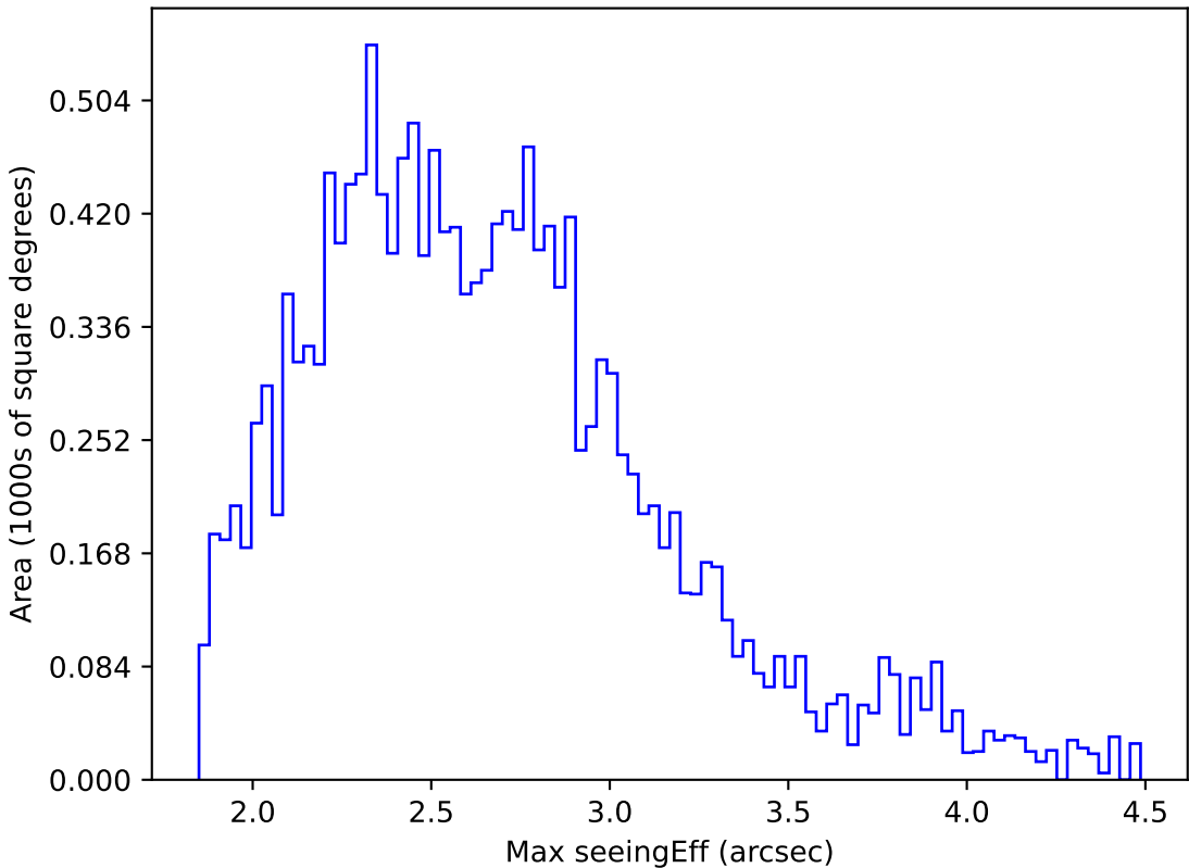
too_elab_r256_d3_griz_v3.4_10yrs WFD r band: Max seeingEff
