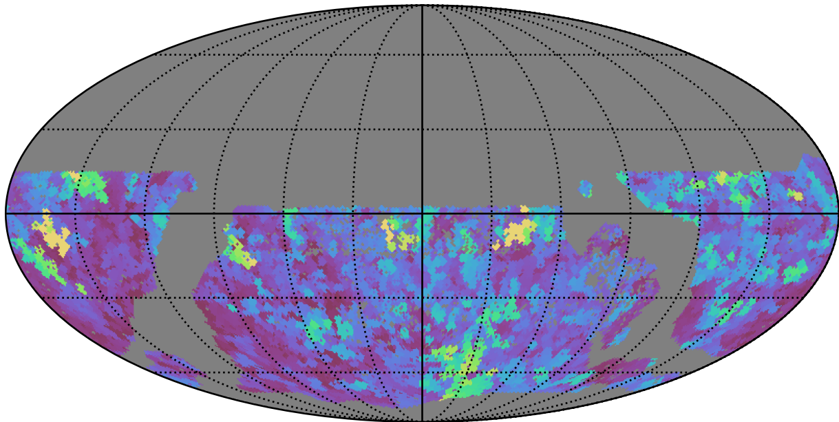
too_elab_r256_d3_griz_v3.4_10yrs WFD i band: Max seeingEff
