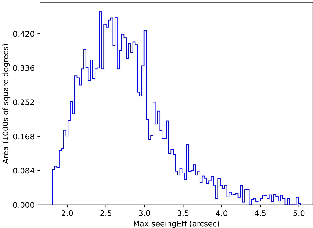
too_elab_r256_d3_griz_v3.4_10yrs WFD i band: Max seeingEff
