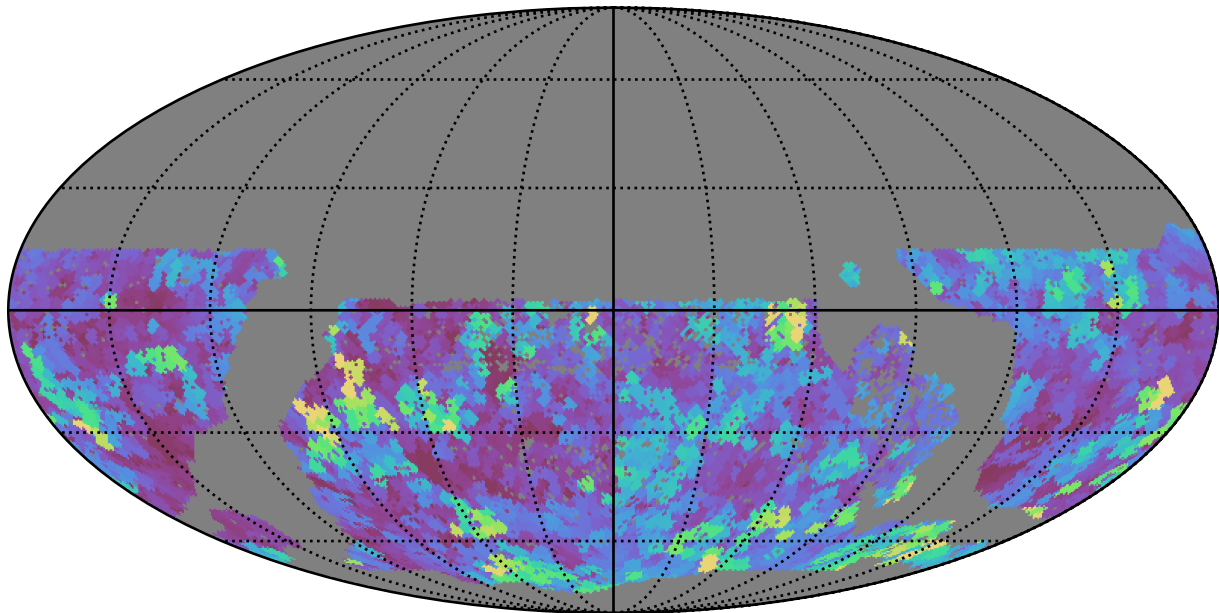
too_elab_r256_d3_griz_v3.4_10yrs WFD g band: Max seeingEff
