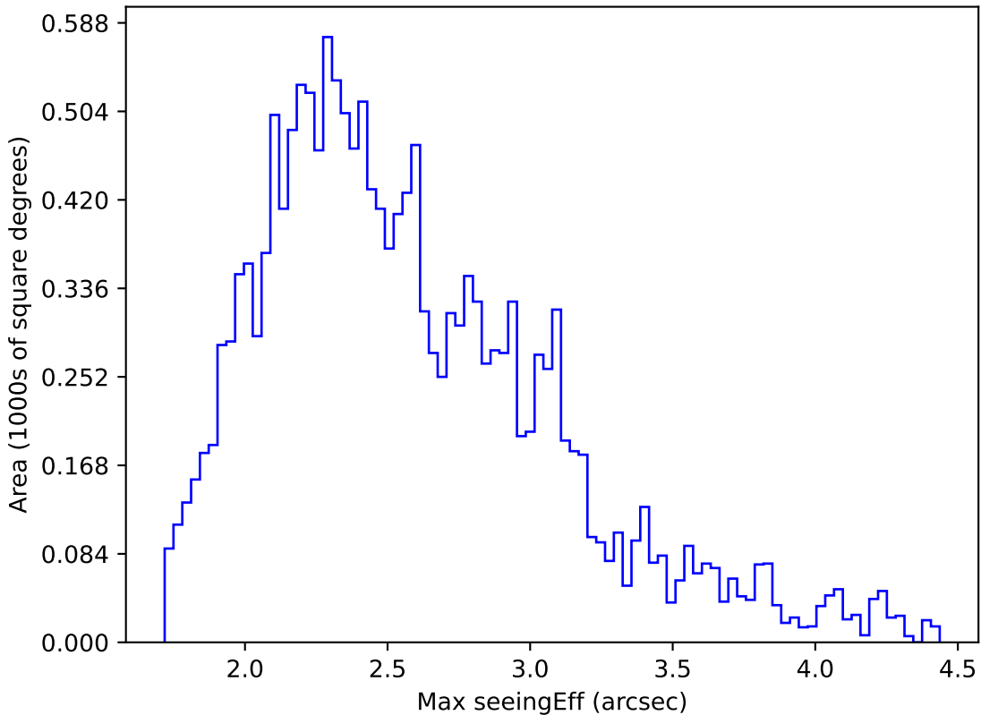
too_elab_r256_d3_griz_v3.4_10yrs WFD g band: Max seeingEff
