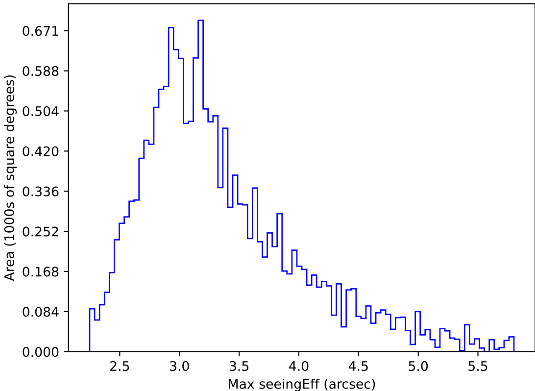
too_elab_r256_d3_griz_v3.4_10yrs WFD all bands: Max seeingEff
