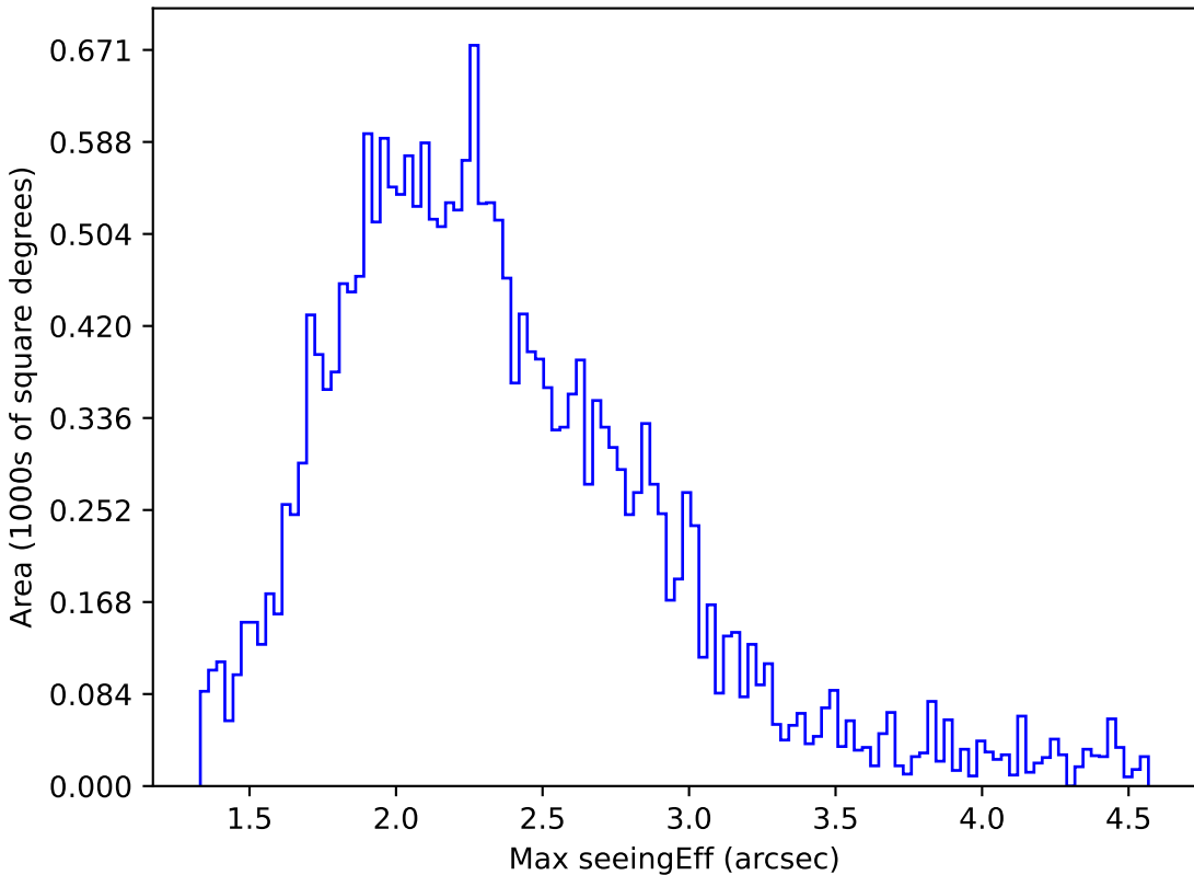
too_elab_r256_d3_griz_v3.4_10yrs All sky y band: Max seeingEff
