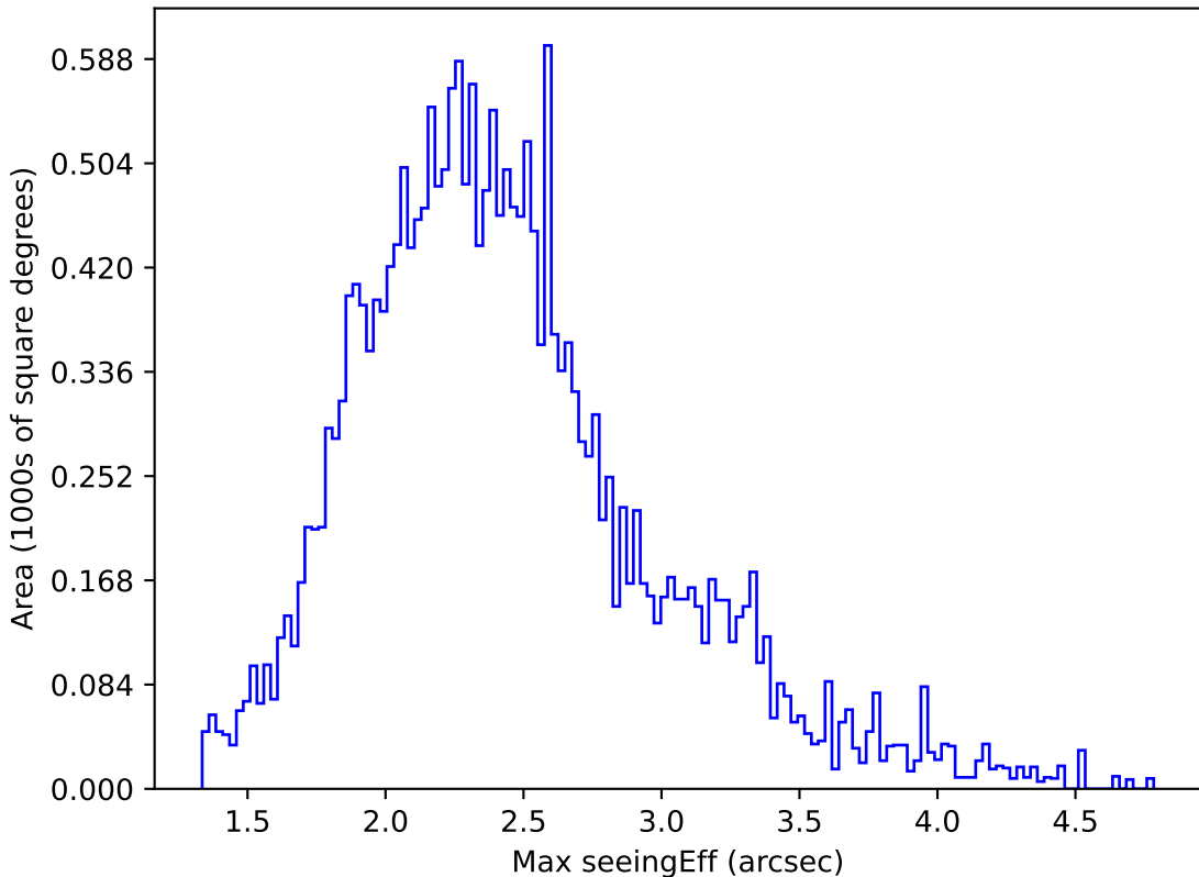
too_elab_r256_d3_griz_v3.4_10yrs All sky u band: Max seeingEff
