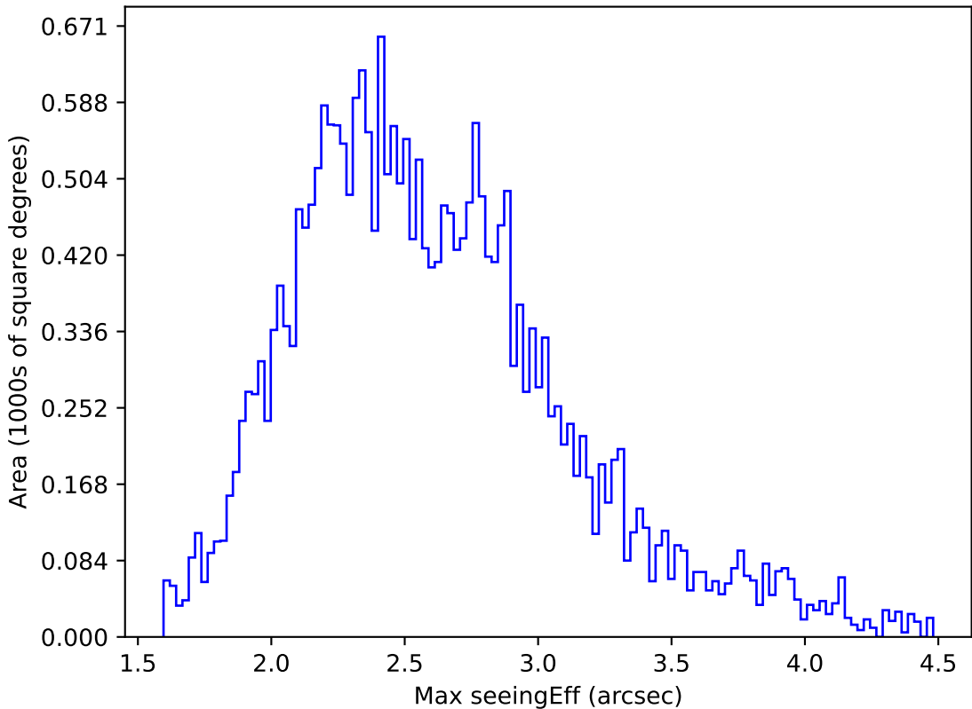
too_elab_r256_d3_griz_v3.4_10yrs All sky r band: Max seeingEff
