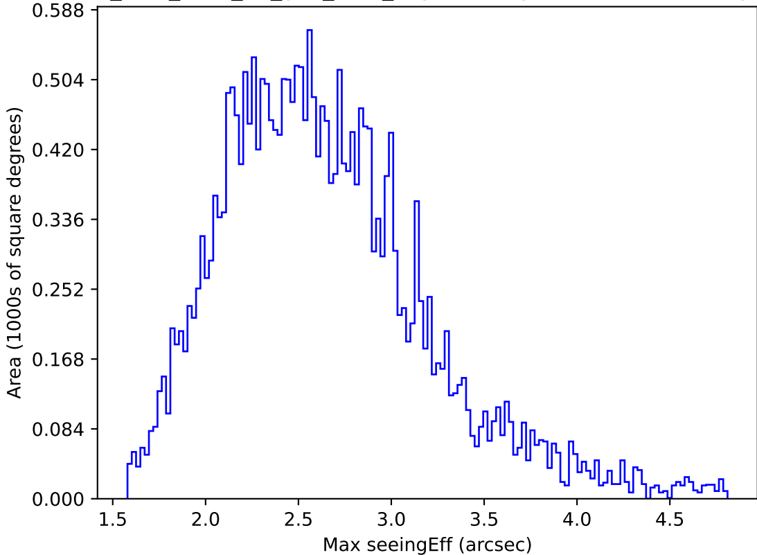
too_elab_r256_d3_griz_v3.4_10yrs All sky i band: Max seeingEff
