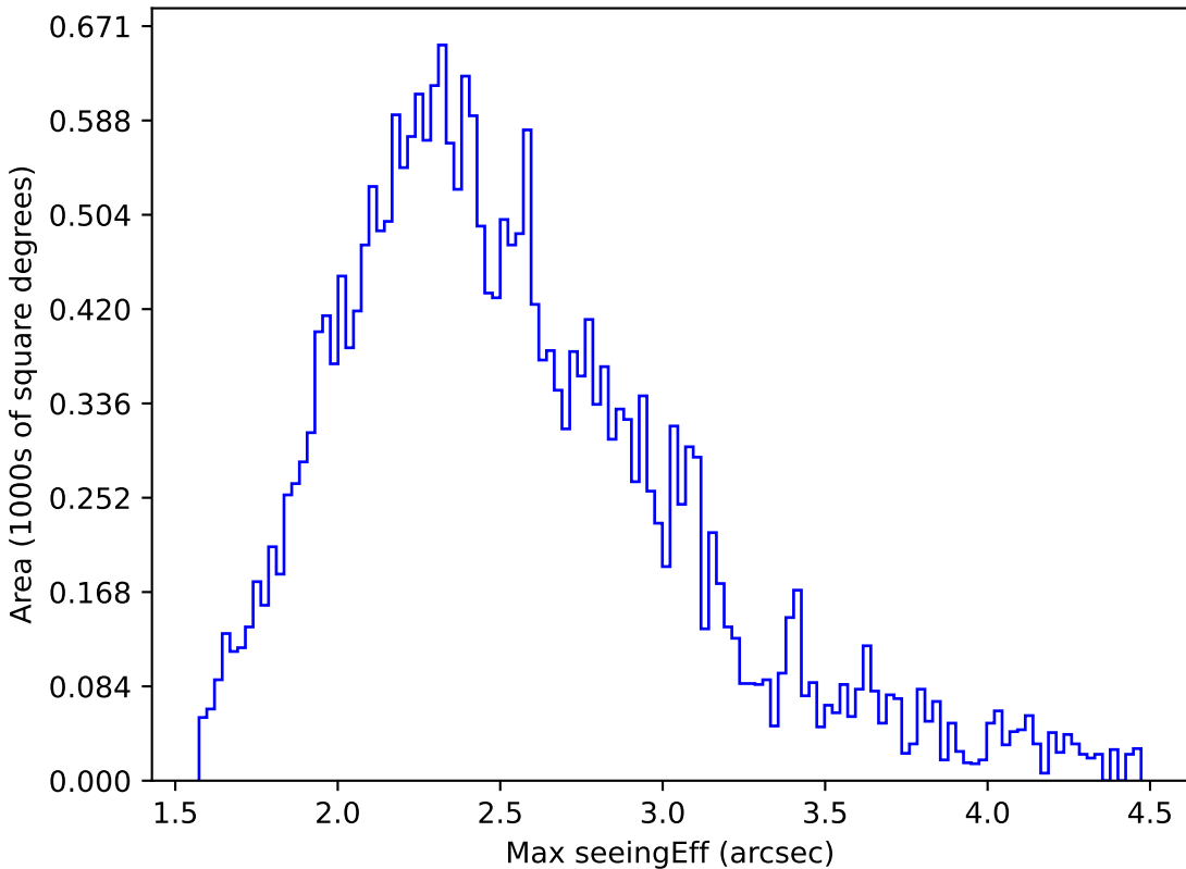
too_elab_r256_d3_griz_v3.4_10yrs All sky g band: Max seeingEff
