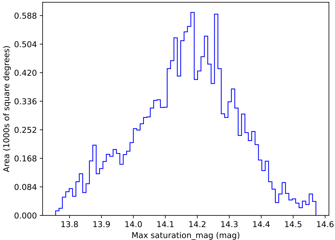
too_elab_r256_d3_griz_v3.4_10yrs WFD y band: Max saturation_mag
