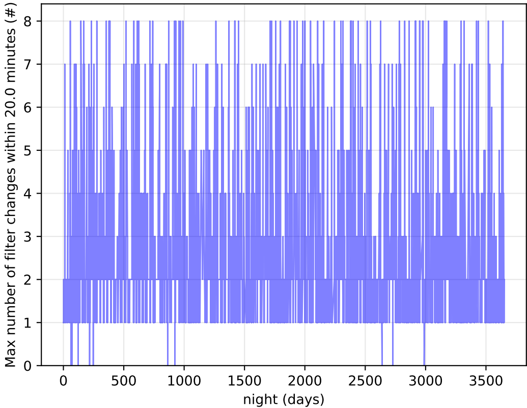
too_elab_r256_d3_griz_v3.4_10yrs Per Night: Max number of filter changes within 20.0 minutes
