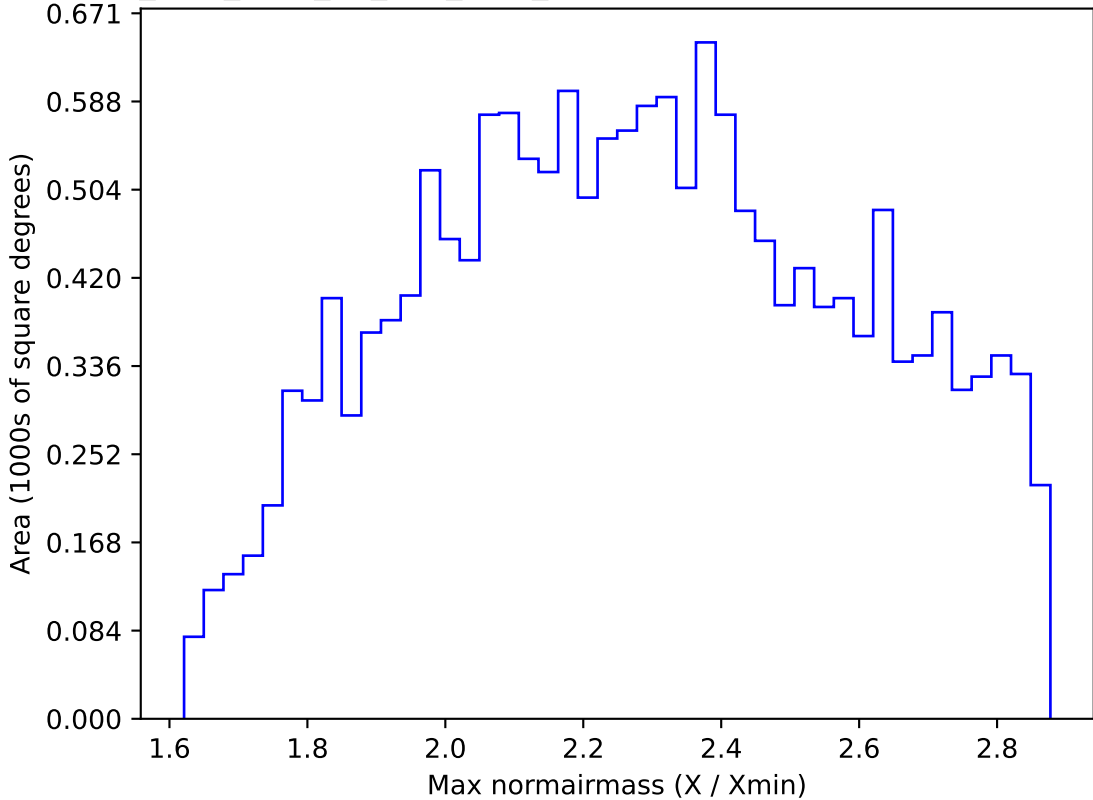
too_elab_r256_d3_griz_v3.4_10yrs WFD z band: Max normairmass
