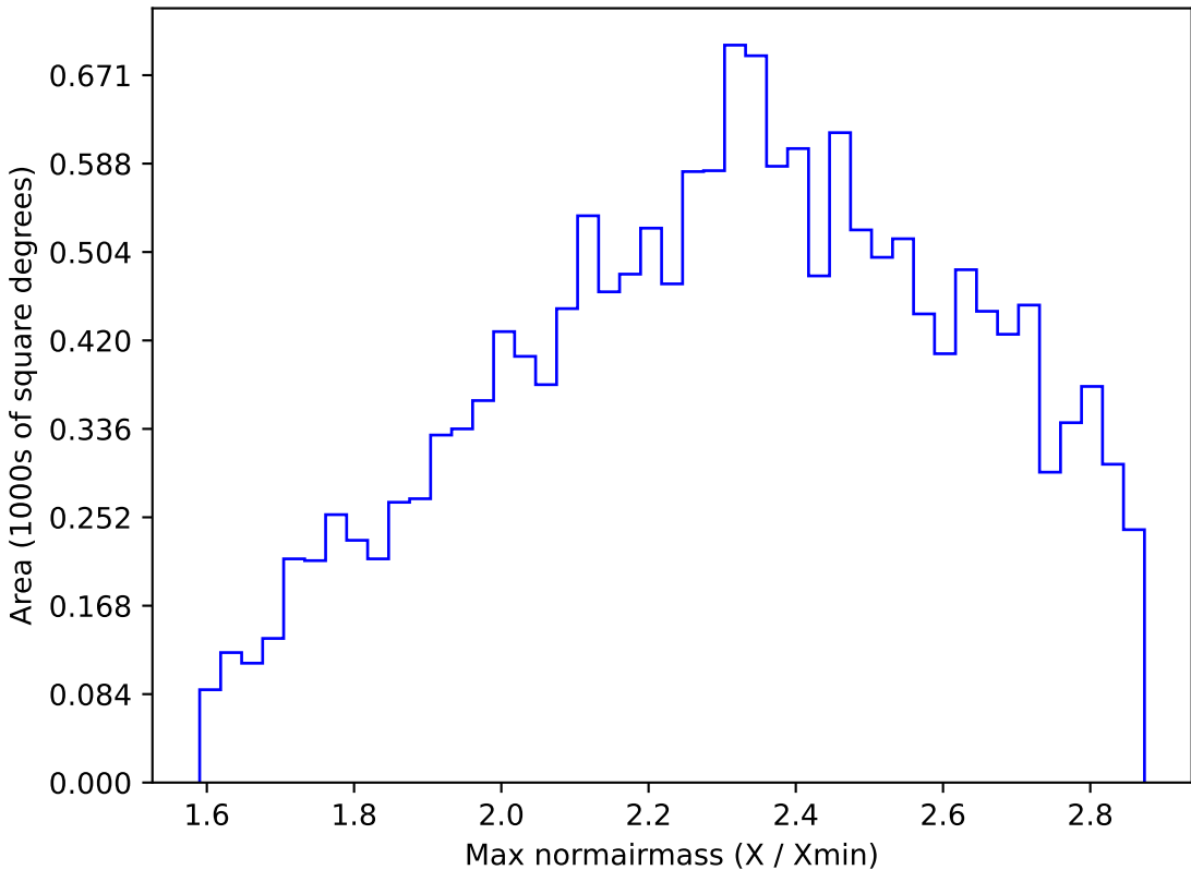
too_elab_r256_d3_griz_v3.4_10yrs WFD i band: Max normairmass
