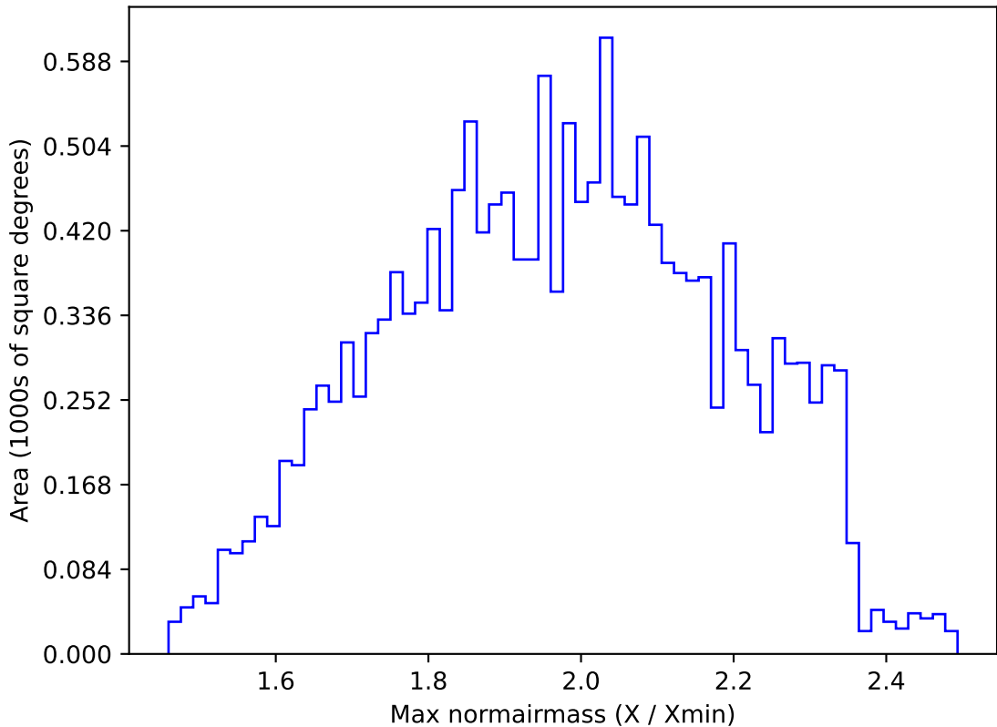
too_elab_r256_d3_griz_v3.4_10yrs WFD g band: Max normairmass
