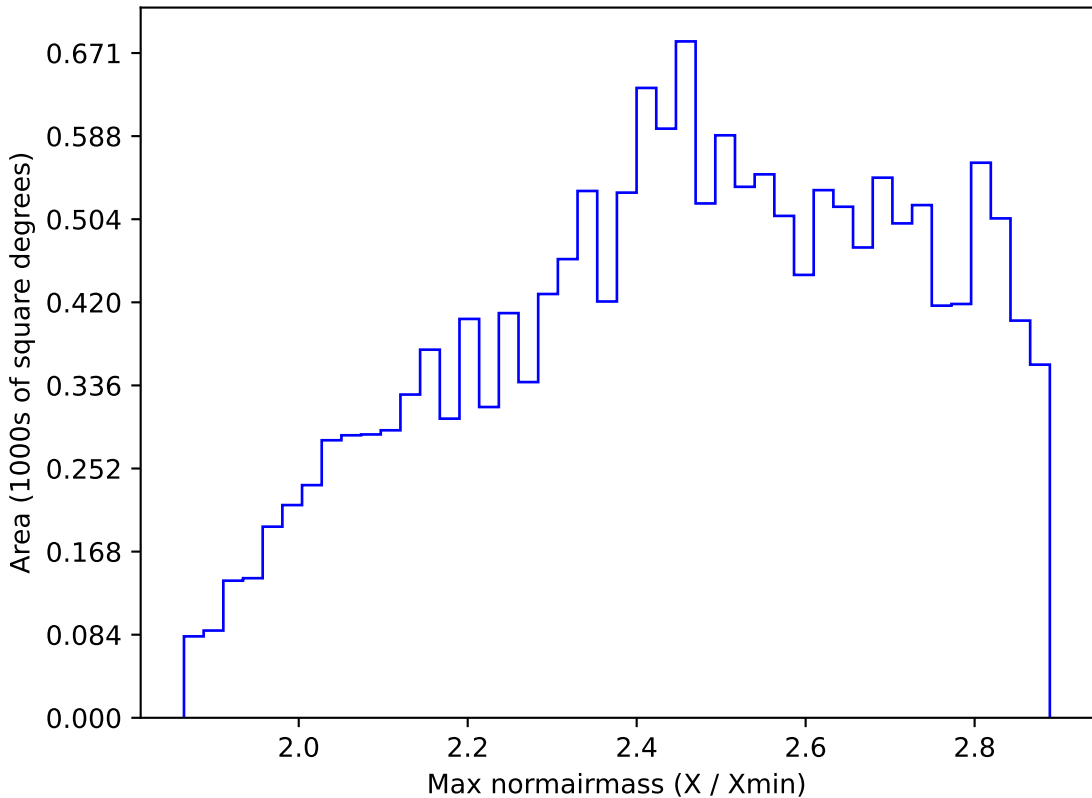
too_elab_r256_d3_griz_v3.4_10yrs WFD all bands: Max normairmass
