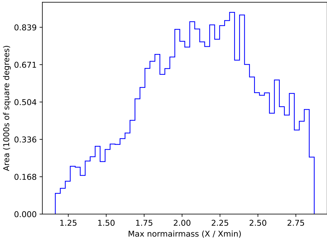
too_elab_r256_d3_griz_v3.4_10yrs All sky z band: Max normairmass
