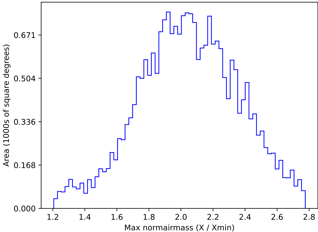
too_elab_r256_d3_griz_v3.4_10yrs All sky y band: Max normairmass
