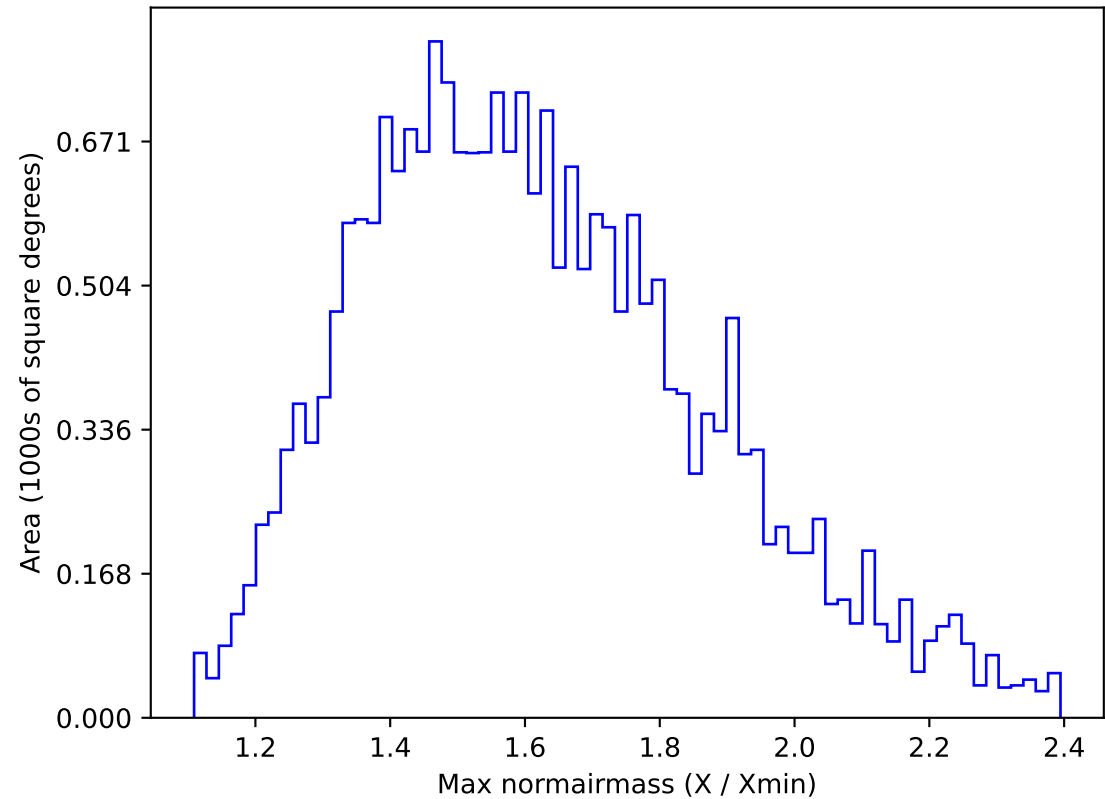
too_elab_r256_d3_griz_v3.4_10yrs All sky u band: Max normairmass
