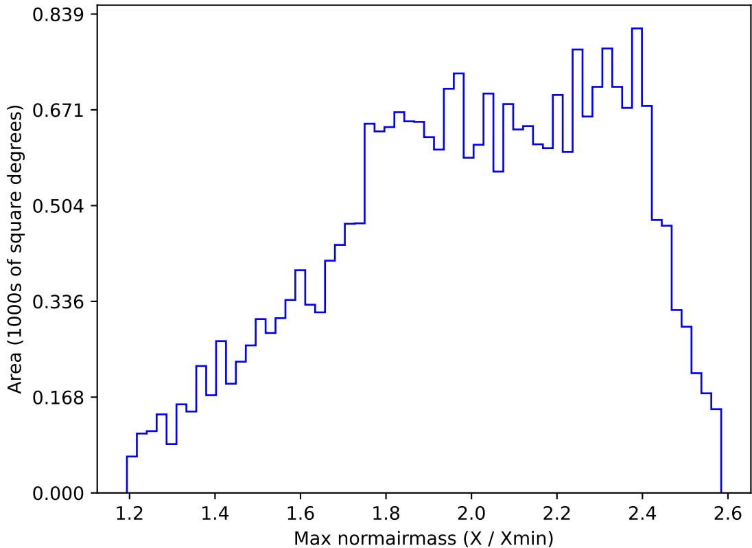
too_elab_r256_d3_griz_v3.4_10yrs All sky r band: Max normairmass
