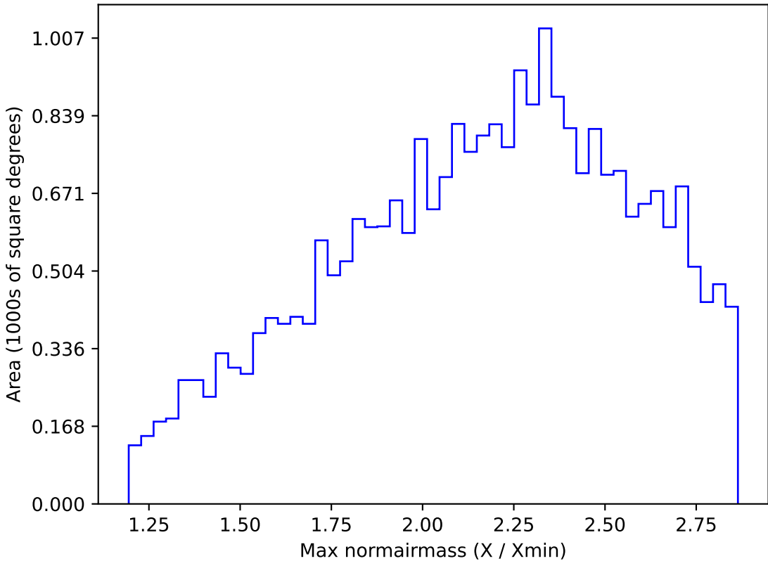
too_elab_r256_d3_griz_v3.4_10yrs All sky i band: Max normairmass
