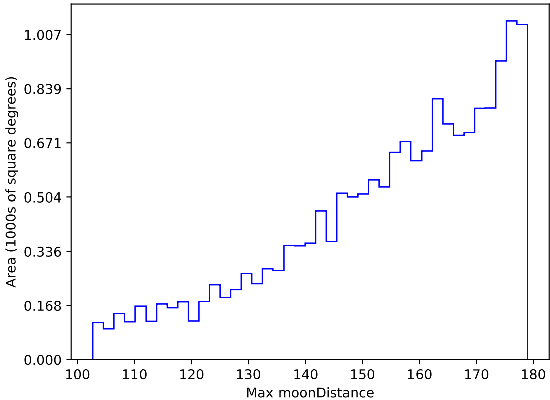
too_elab_r256_d3_griz_v3.4_10yrs WFD z band: Max moonDistance
