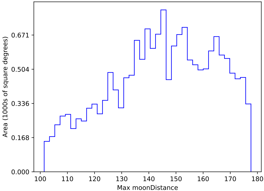
too_elab_r256_d3_griz_v3.4_10yrs WFD y band: Max moonDistance
