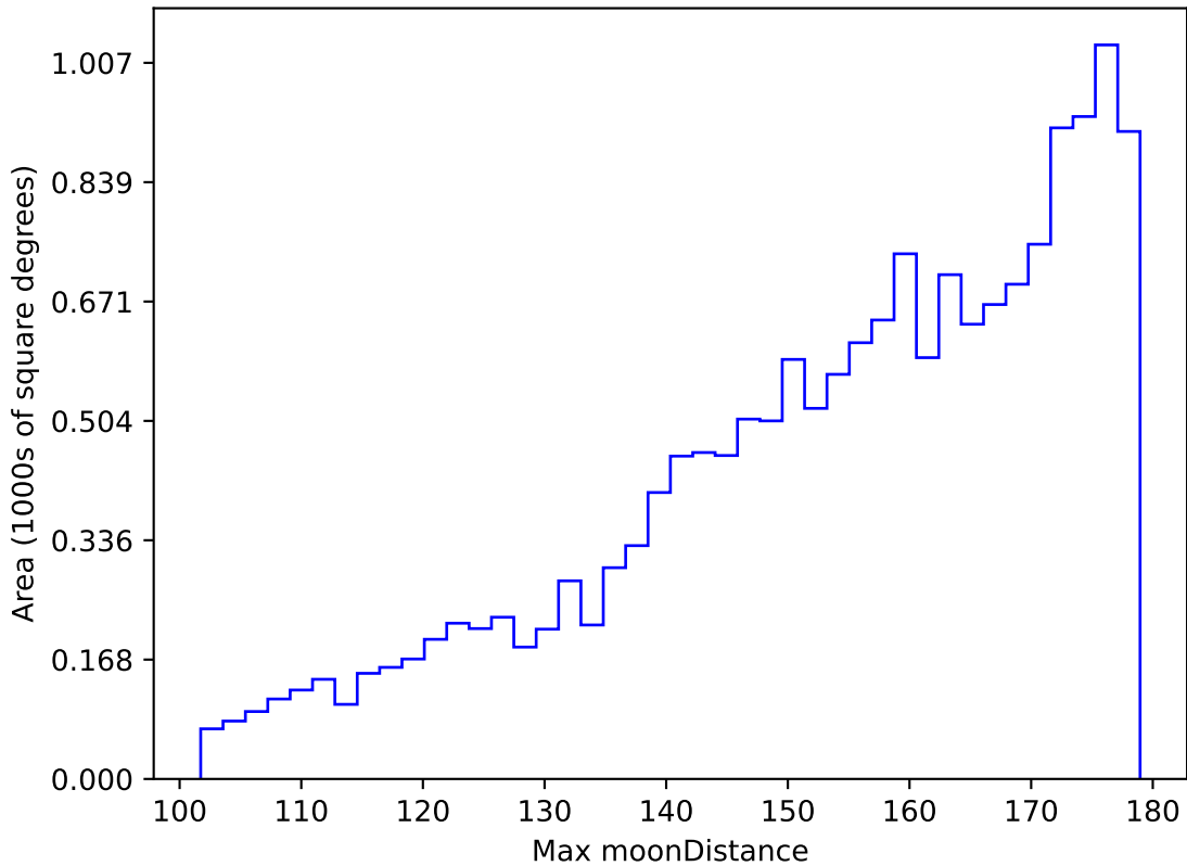
too_elab_r256_d3_griz_v3.4_10yrs WFD u band: Max moonDistance
