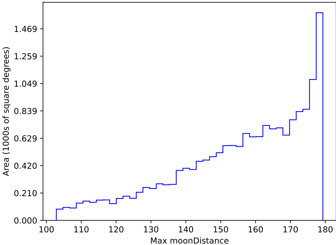
too_elab_r256_d3_griz_v3.4_10yrs WFD r band: Max moonDistance
