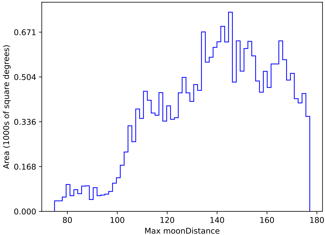
too_elab_r256_d3_griz_v3.4_10yrs All sky y band: Max moonDistance
