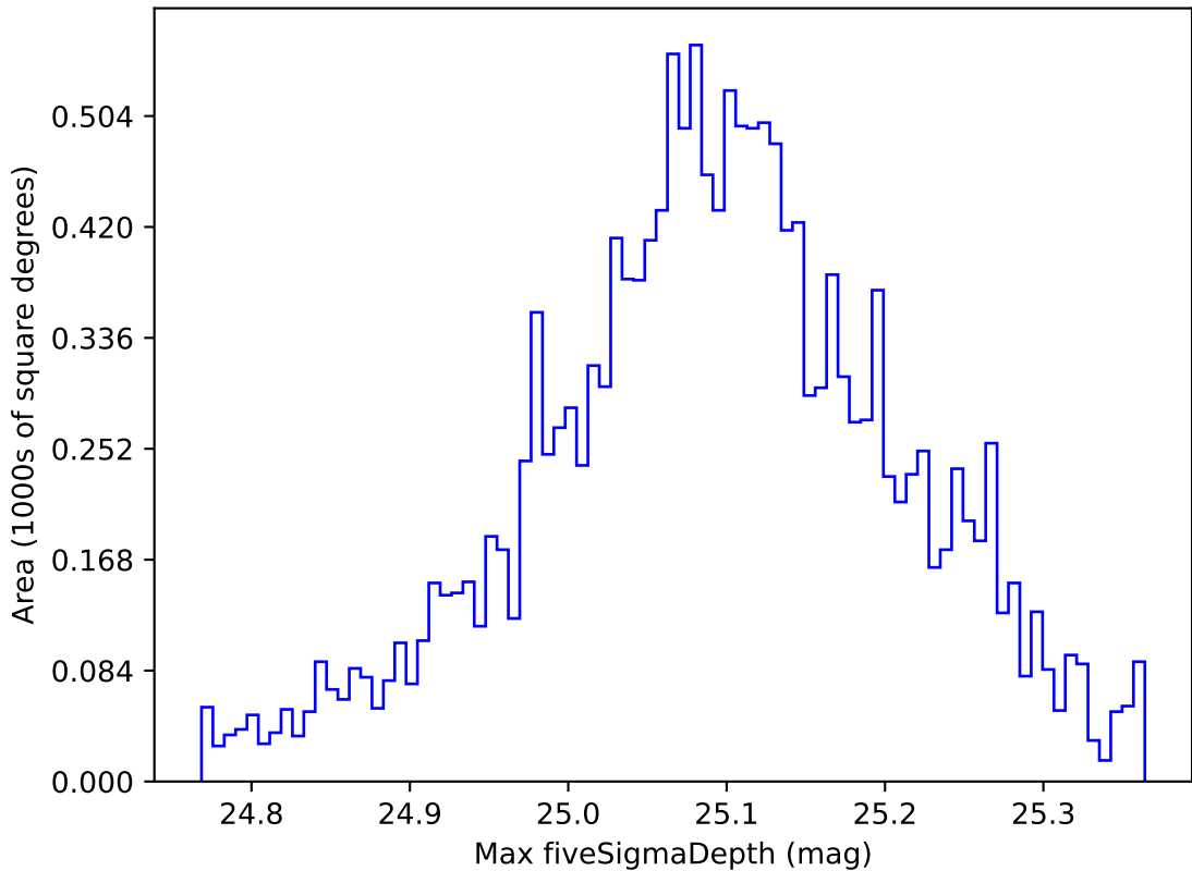
too_elab_r256_d3_griz_v3.4_10yrs WFD g band: Max fiveSigmaDepth
