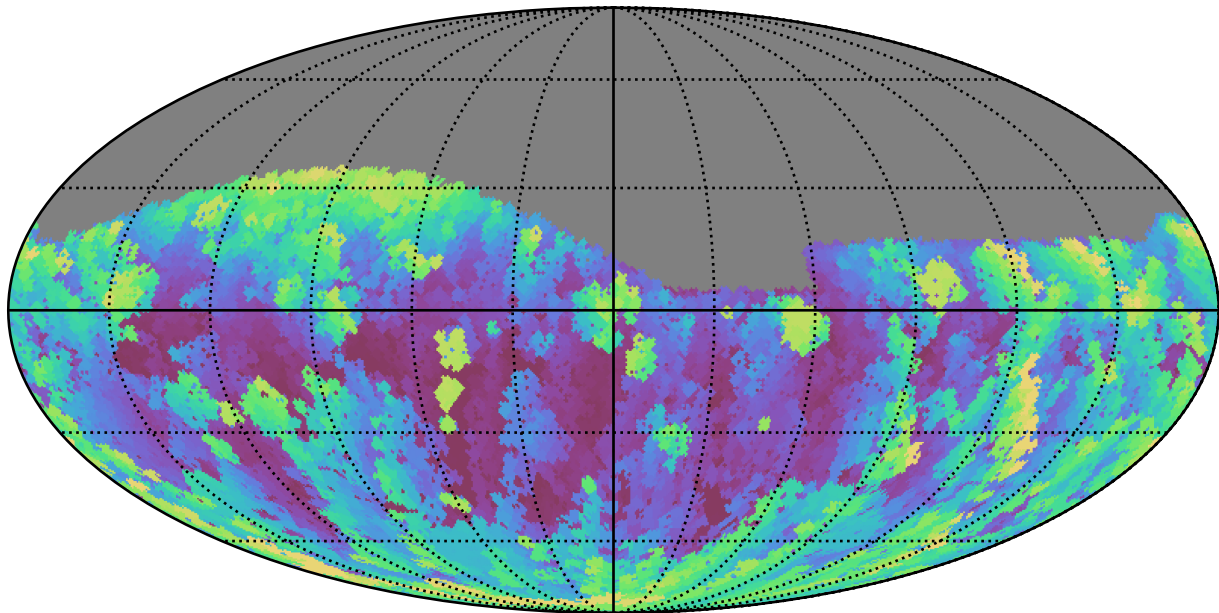
too_elab_r256_d3_griz_v3.4_10yrs Yr 1 g band: Max airmass
