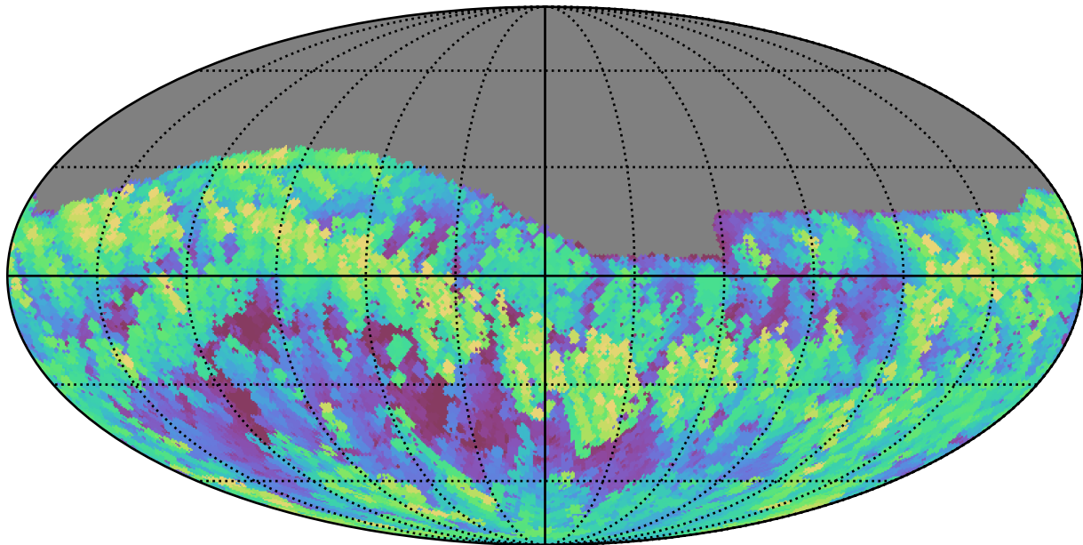
too_elab_r256_d3_griz_v3.4_10yrs Yr 1 all bands: Max airmass
