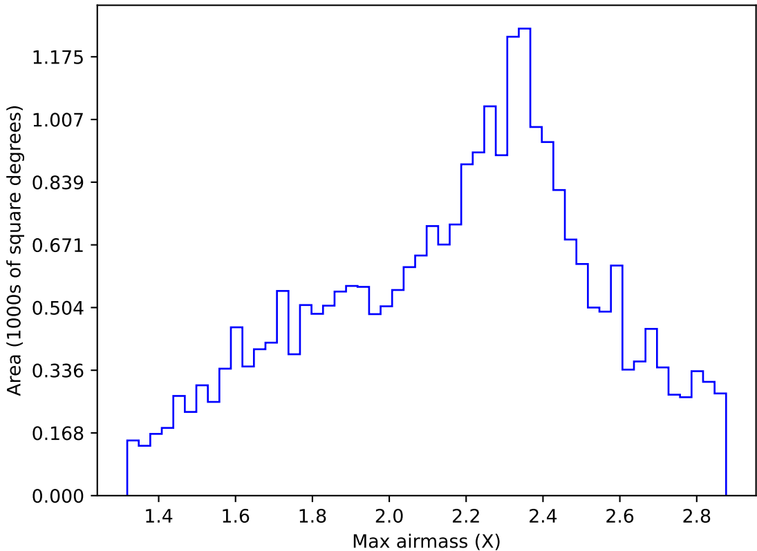
too_elab_r256_d3_griz_v3.4_10yrs Yr 1 all bands: Max airmass
