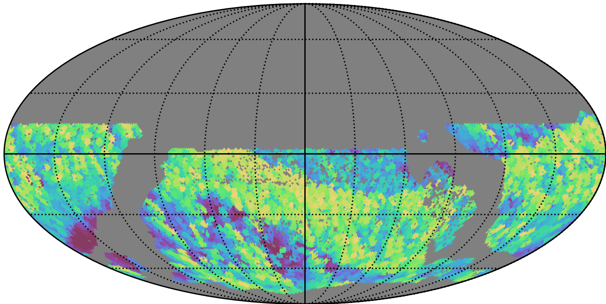
too_elab_r256_d3_griz_v3.4_10yrs WFD i band: Max airmass
