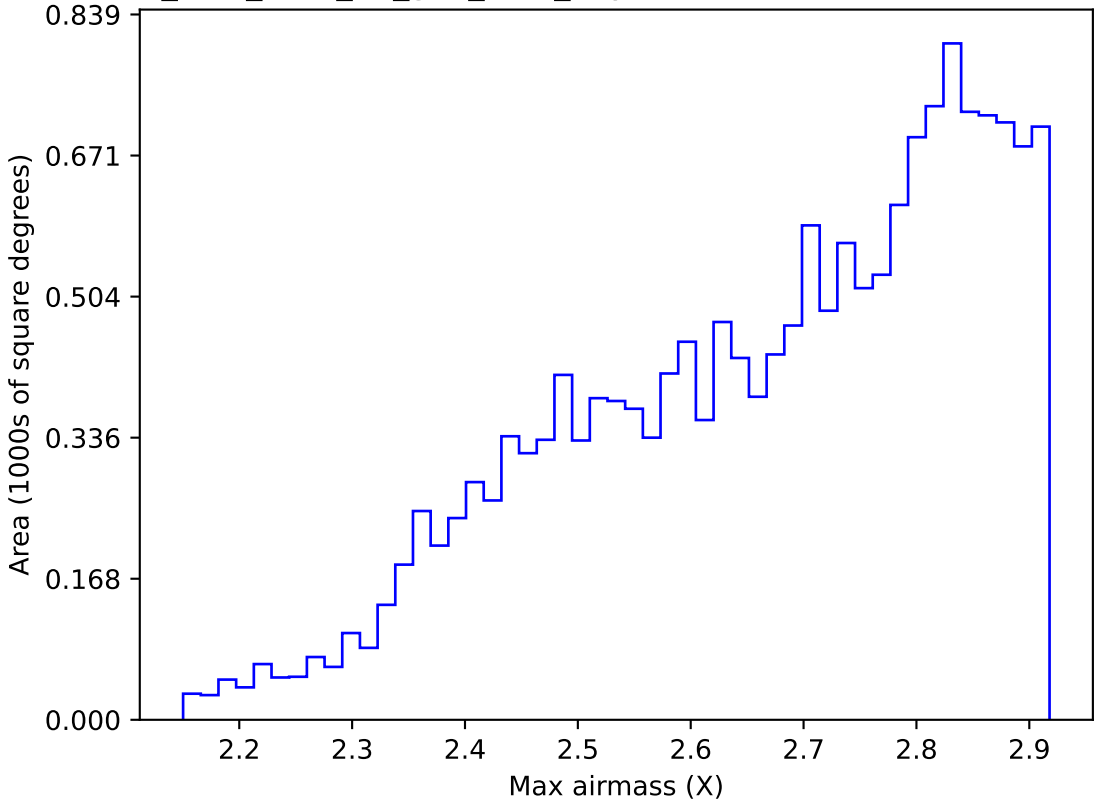
too_elab_r256_d3_griz_v3.4_10yrs WFD all bands: Max airmass
