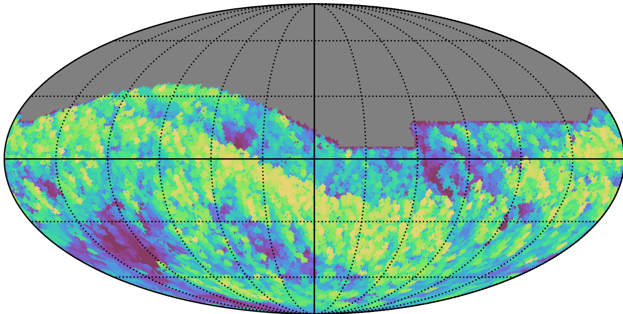
too_elab_r256_d3_griz_v3.4_10yrs All sky z band: Max airmass
