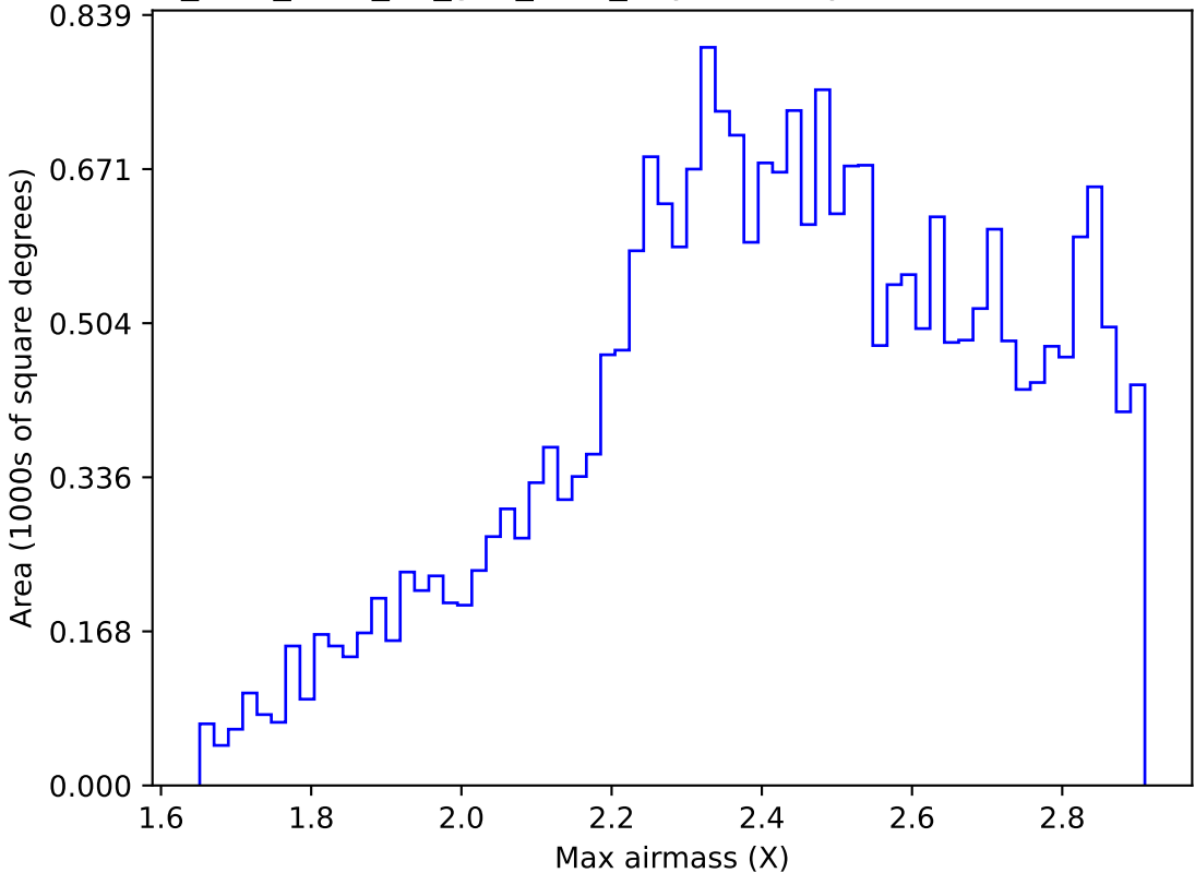
too_elab_r256_d3_griz_v3.4_10yrs All sky z band: Max airmass
