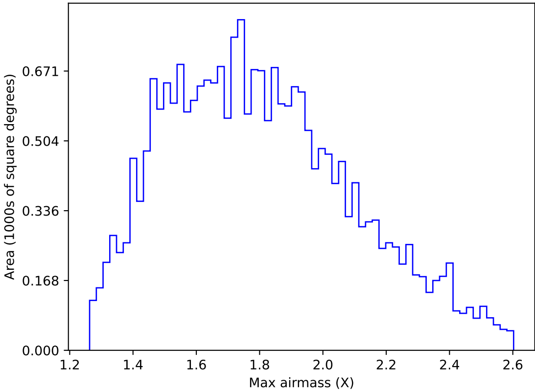
too_elab_r256_d3_griz_v3.4_10yrs All sky u band: Max airmass
