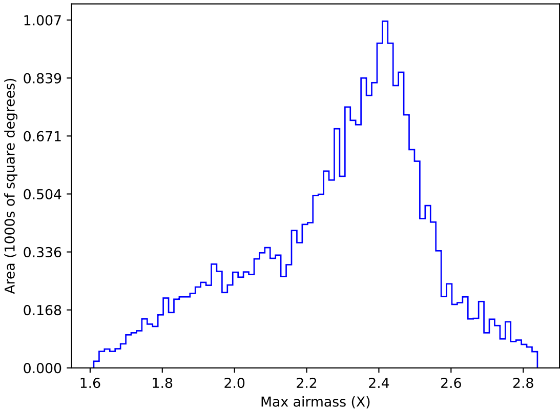
too_elab_r256_d3_griz_v3.4_10yrs All sky r band: Max airmass
