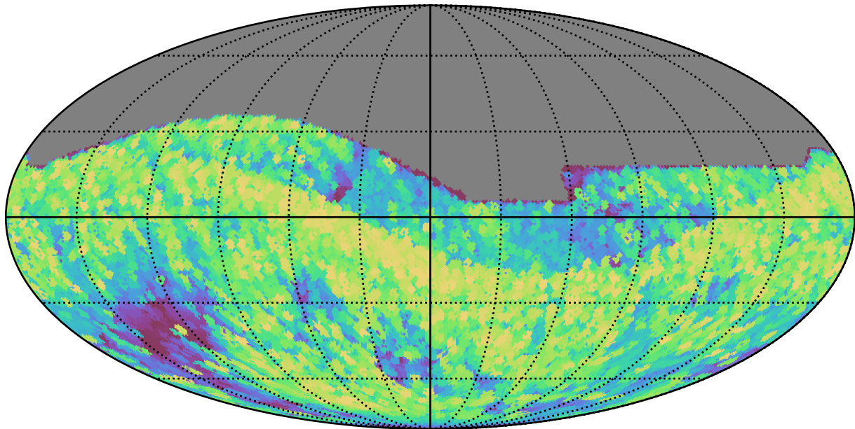
too_elab_r256_d3_griz_v3.4_10yrs All sky all bands: Max airmass
