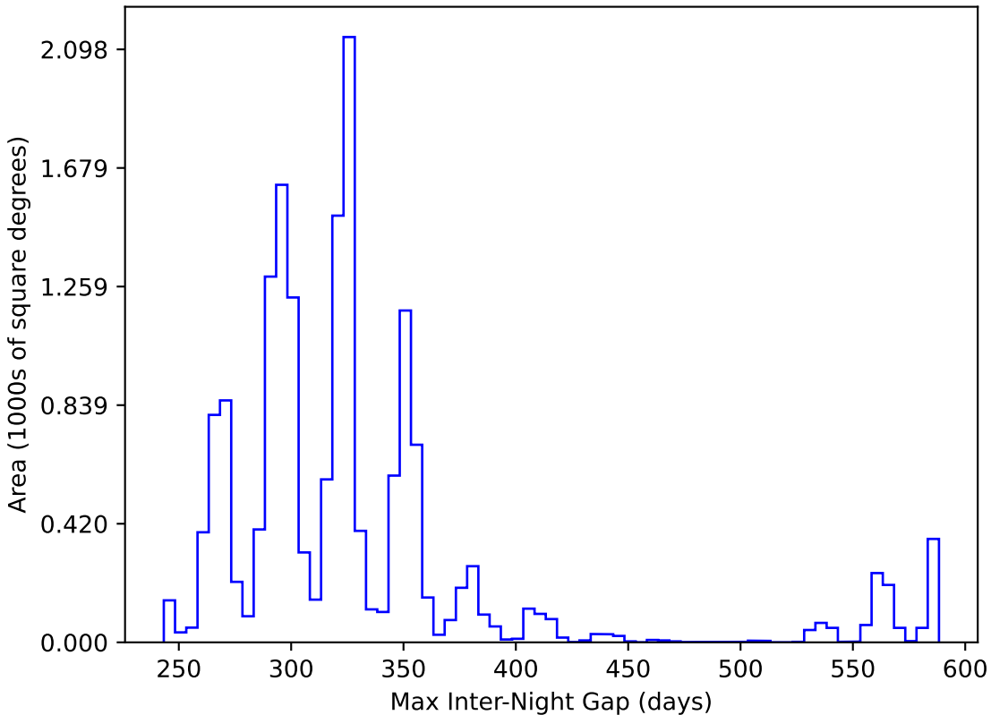
too_elab_r256_d3_griz_v3.4_10yrs WFD y band: Max Inter-Night Gap
