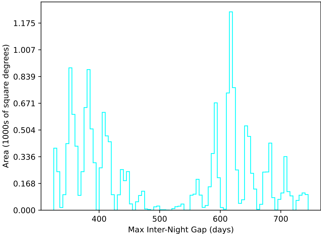
too_elab_r256_d3_griz_v3.4_10yrs WFD u band: Max Inter-Night Gap
