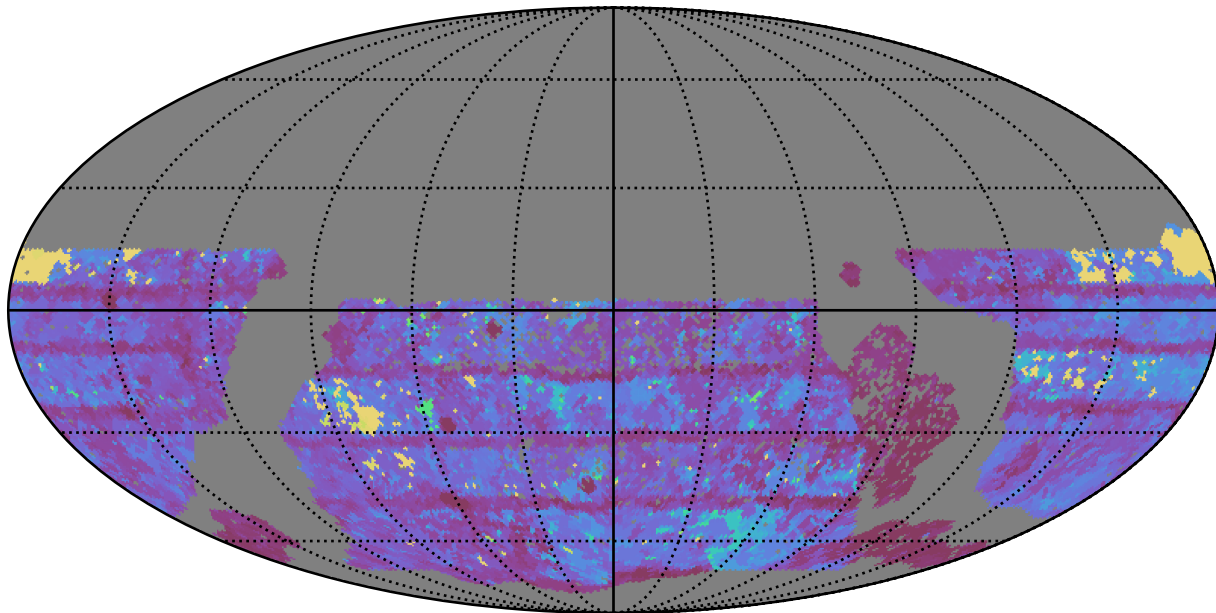
too_elab_r256_d3_griz_v3.4_10yrs WFD r band: Max Inter-Night Gap
