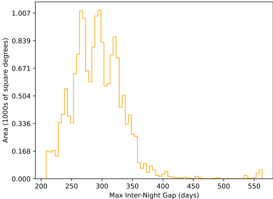
too_elab_r256_d3_griz_v3.4_10yrs WFD r band: Max Inter-Night Gap
