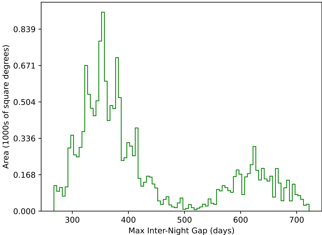
too_elab_r256_d3_griz_v3.4_10yrs WFD g band: Max Inter-Night Gap
