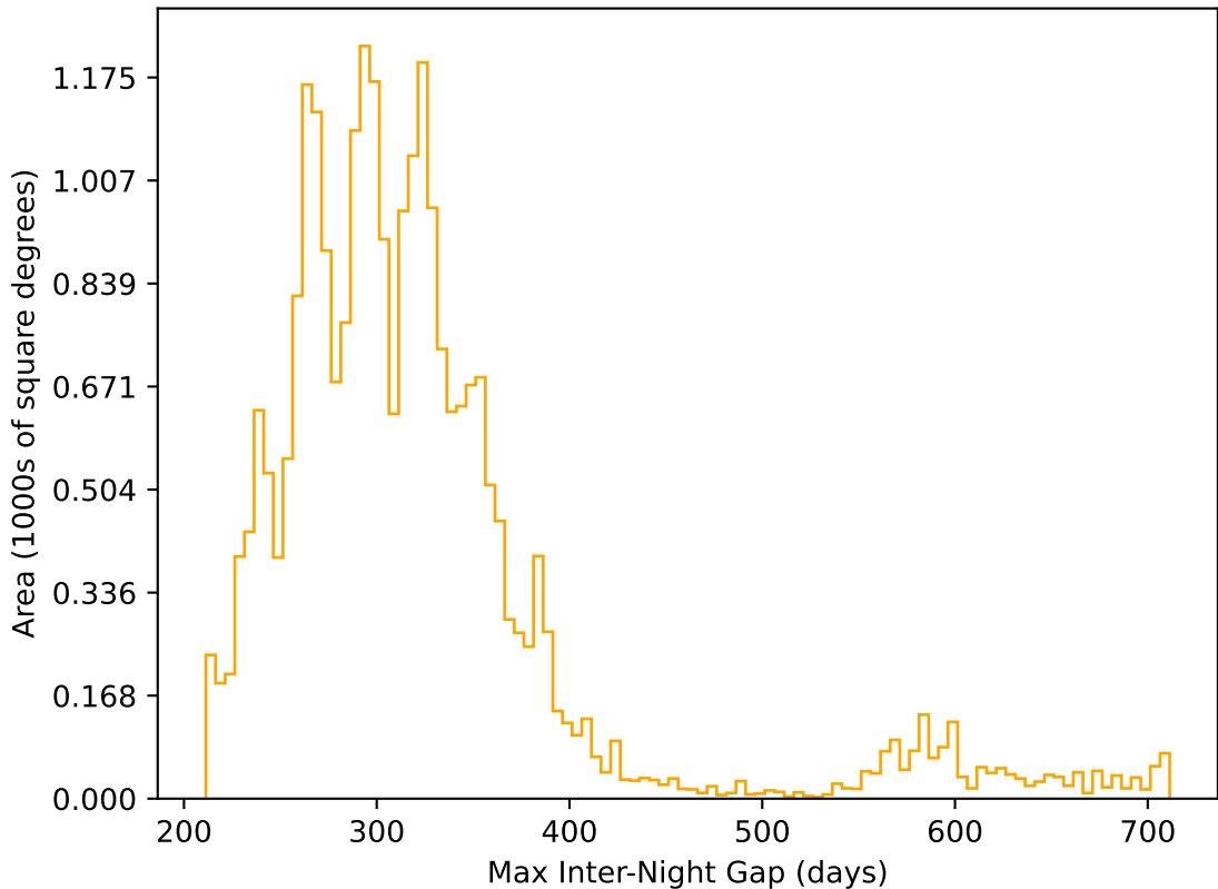
too_elab_r256_d3_griz_v3.4_10yrs All sky r band: Max Inter-Night Gap
