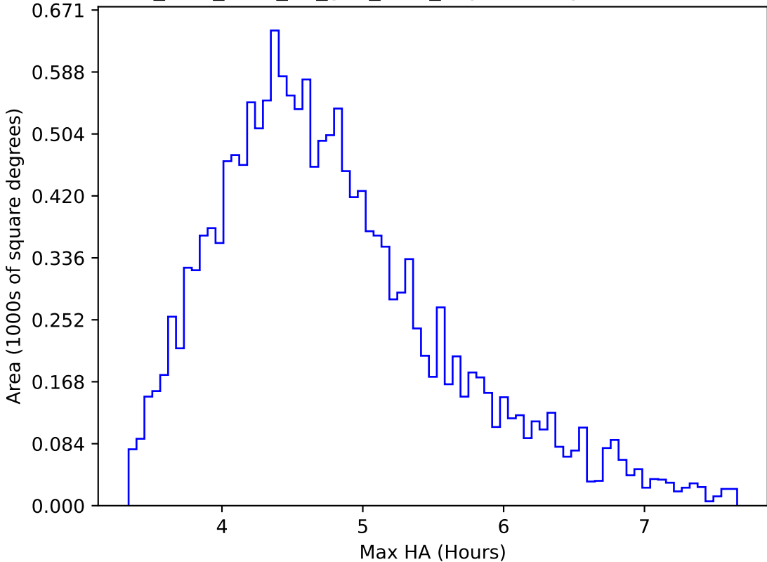
too_elab_r256_d3_griz_v3.4_10yrs WFD y band: Max HA
