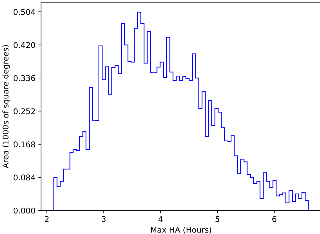
too_elab_r256_d3_griz_v3.4_10yrs WFD u band: Max HA
